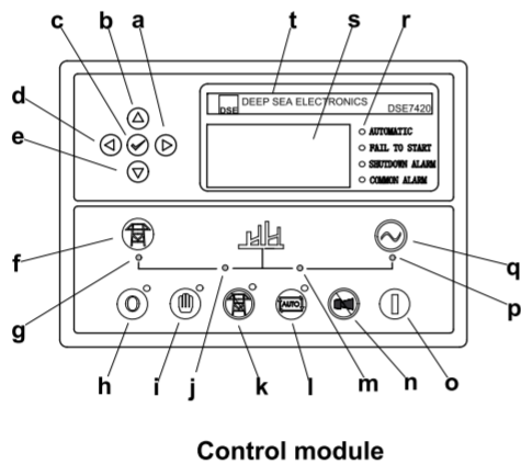
Control module
